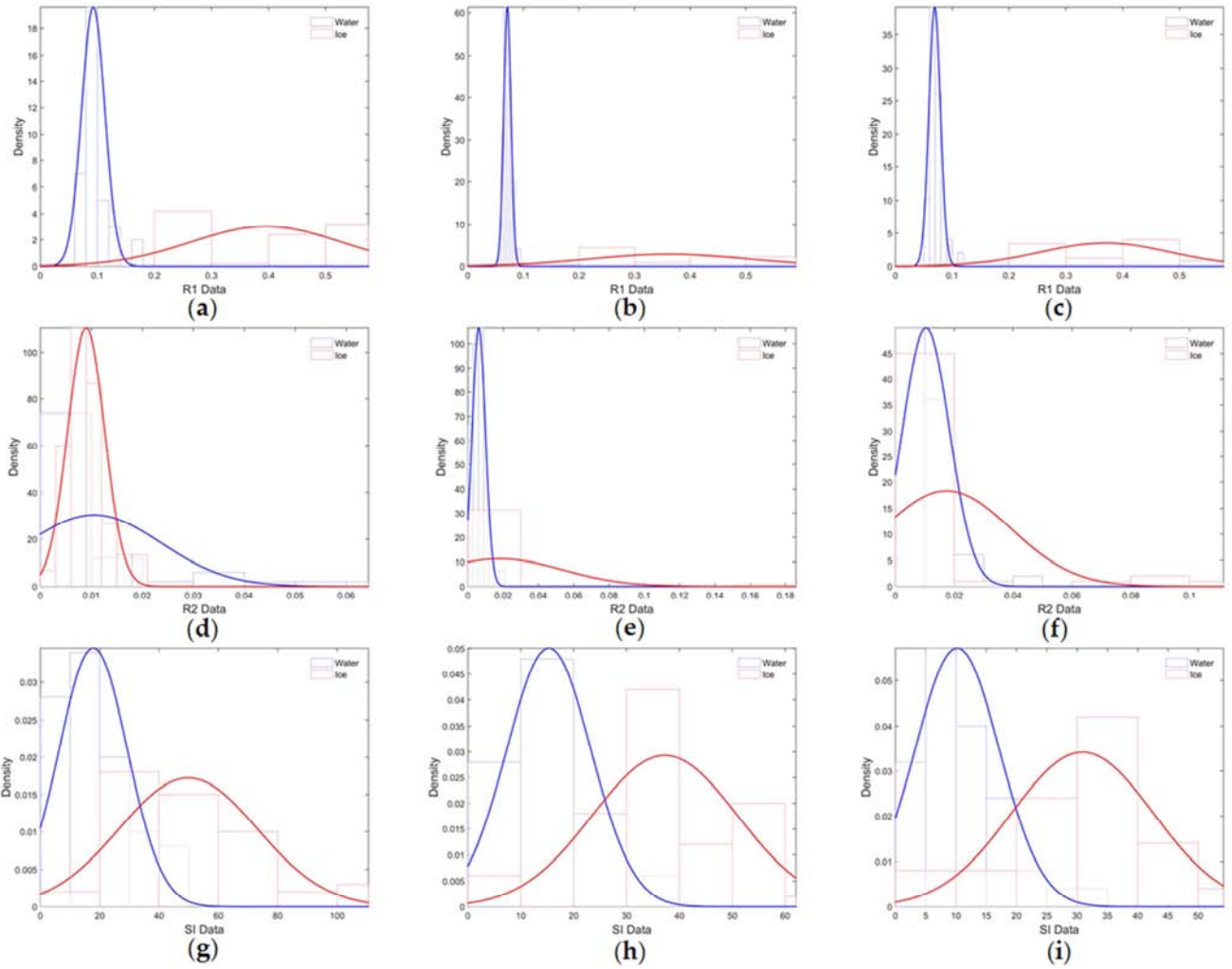
Figure 3. Probability distribution functions of water (blue) and ice (red) at 1430, 1730, 2030 UTC on February 28, 2015; (top) distribution of 0.64 \mu\text{m} refl; (middle) distribution of 3.9 \mu\text{m} refl; (bottom) distribution of MISI.
