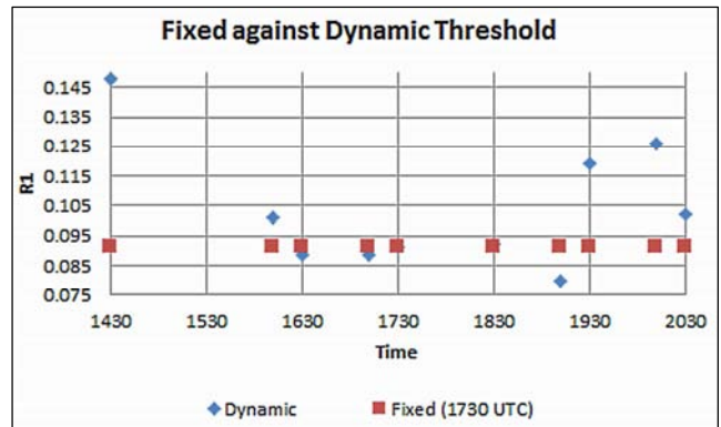
Figure 5. Fixed threshold against dynamic threshold versus acquisition times.
